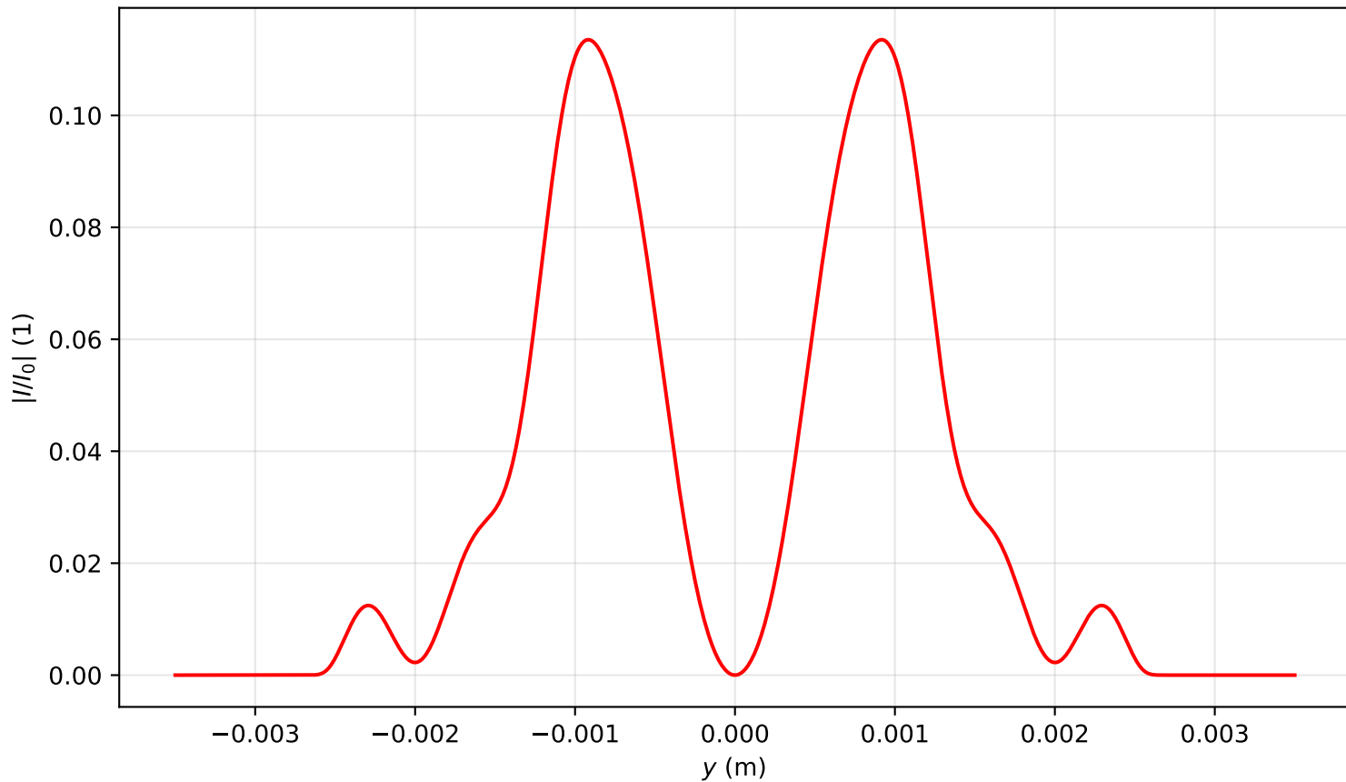
Intensity profile I(x=0, y, z=3.662)/I_0 , \text{Pin}=4.0\text{Pcr} , artificial time
